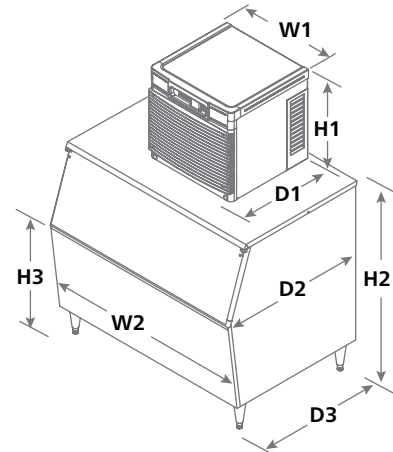
Back view — air-cooled, top mount
